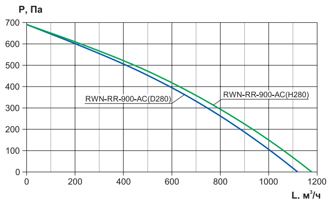
RWN-RR-900-AC-Compact
