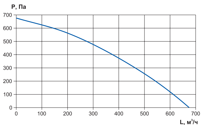
RWN-RR-500-AC-Vertical
