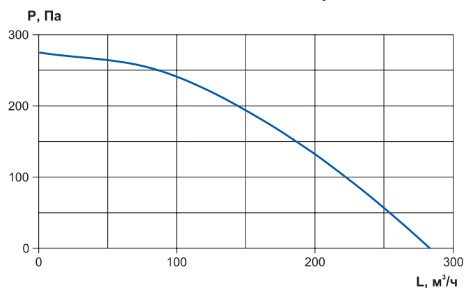
RWN-RP-400-AC-Compact
