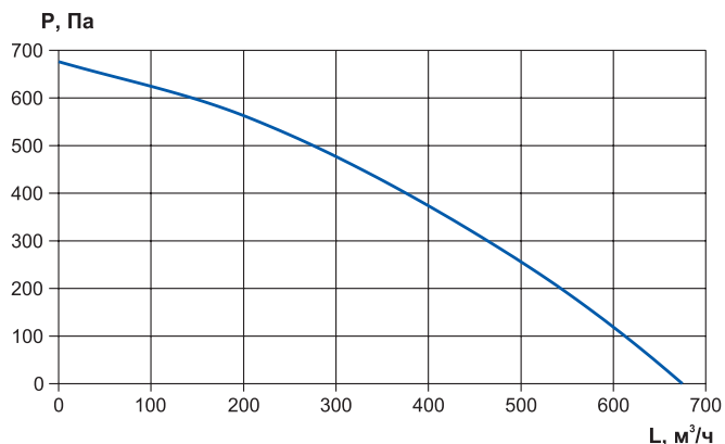
RWN-RR-500-AC-Compact
