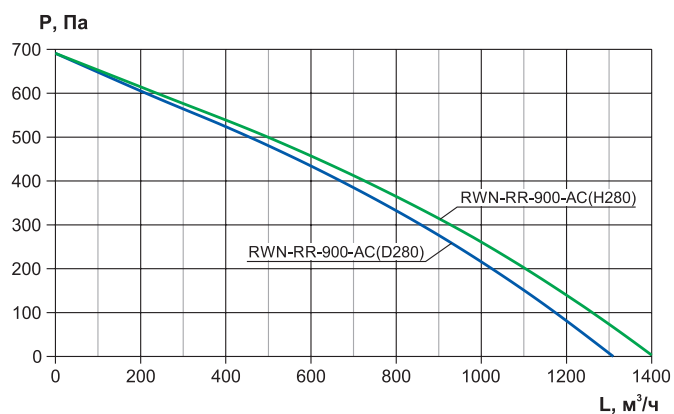
RWN-RR-900-AC-Vertical
