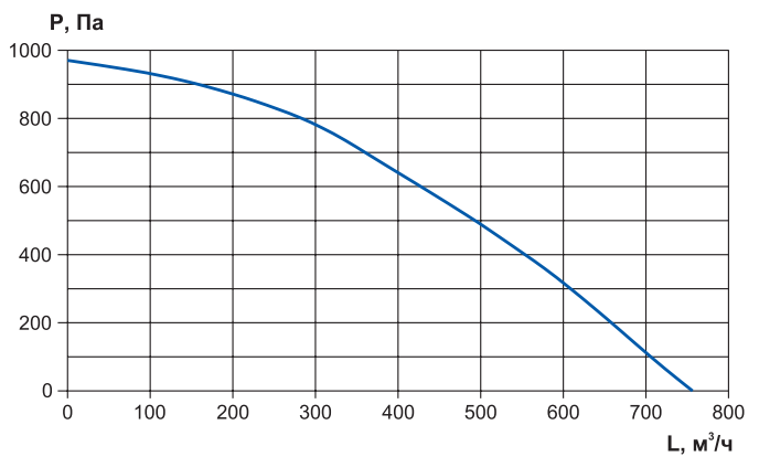
RWN-F-500-EC
