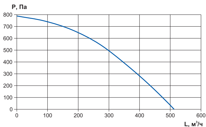
RWN-RP-600-EC-Vertical
