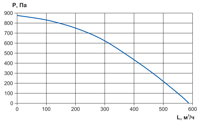
RWN-RR-600-EC-Vertical
