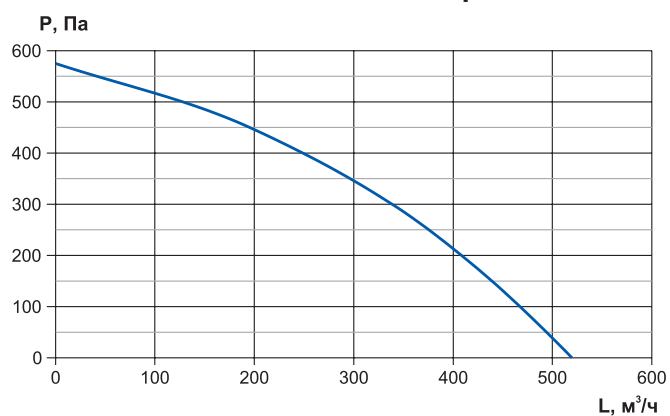
RWN-RP-1500-AC-Compact
