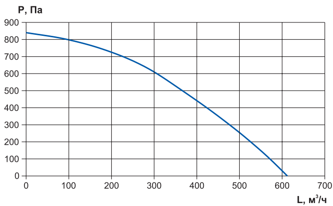
RWN-F-400-EC
