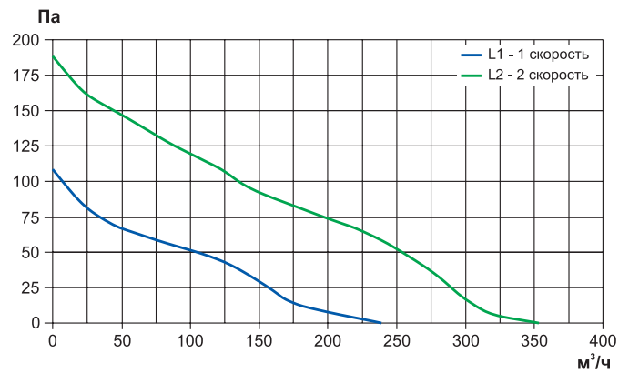
TYPHOON 200 2SP
