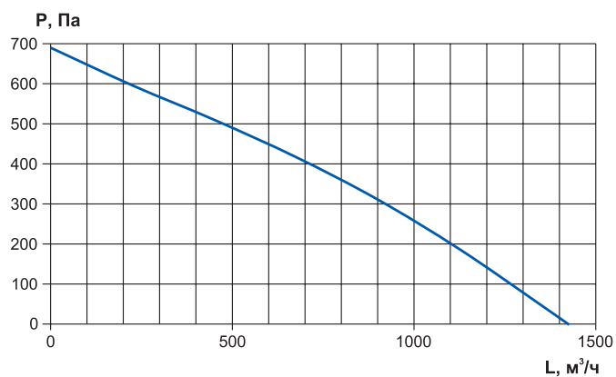
RWN-F-900-AC
