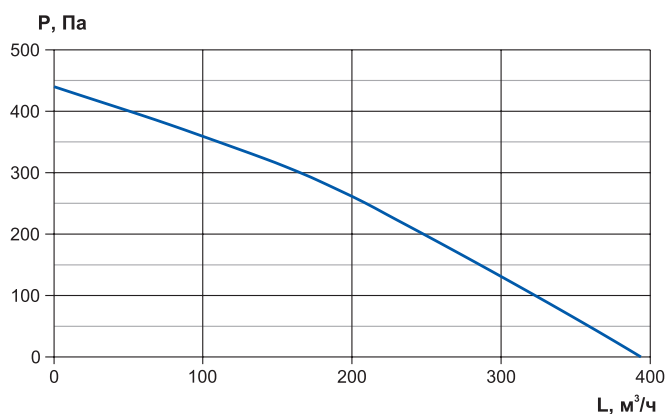
RWN-RP-800-AC-Vertical
