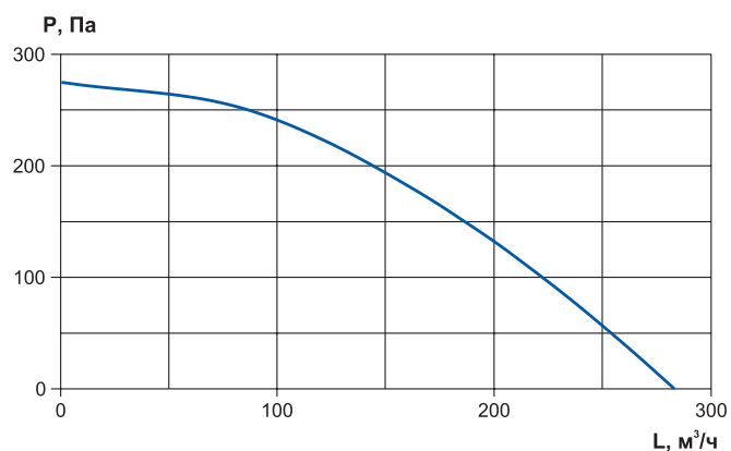
RWN-RP-400-AC-Vertical
