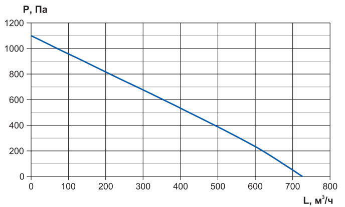
RWN-RR-1300-EC-Vertical
