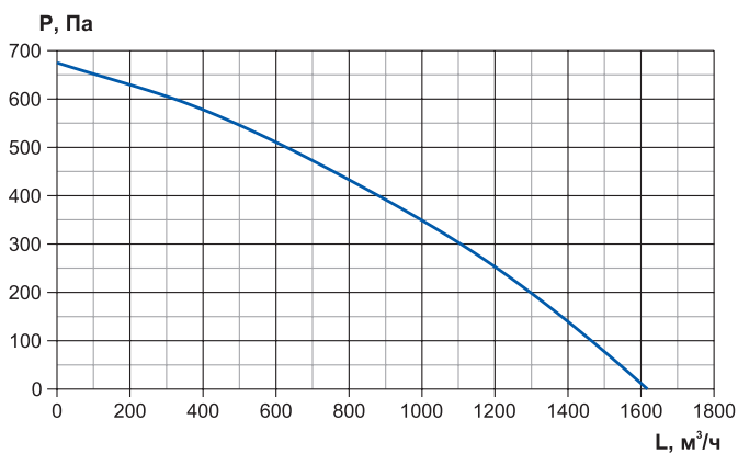
RWN-RP-1500-AC-Vertical
