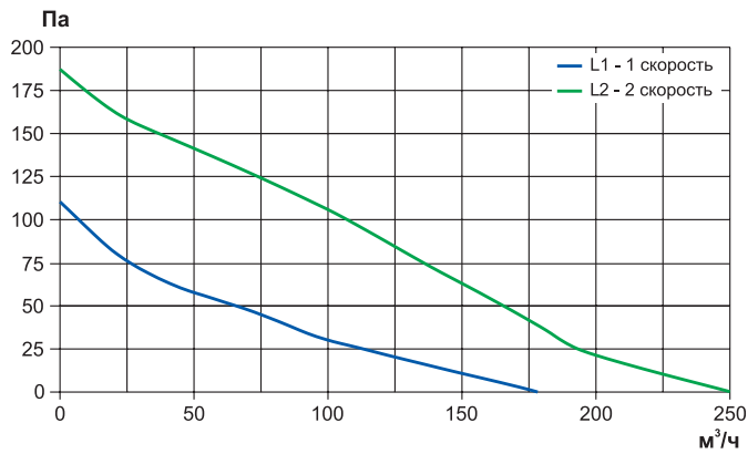
TYPHOON 150/160 2SP
