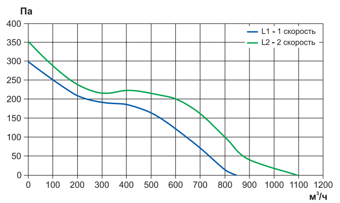
TYPHOON 315 2SP
