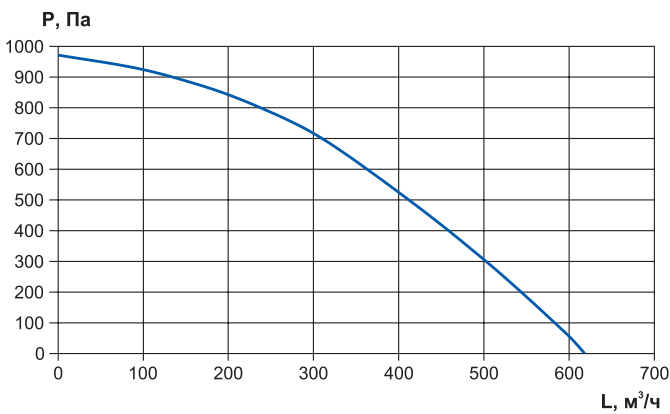
RWN-RR-1000-EC-Vertical
